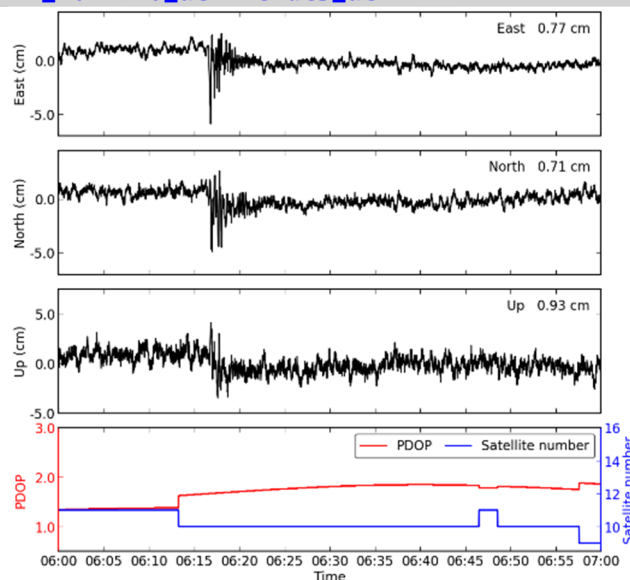
Figure 5-25 Position time series of ac12, 210 day in 2021
