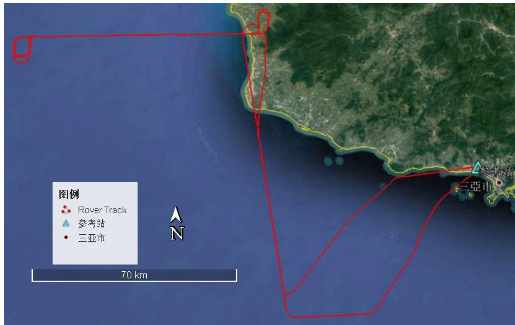
Figure B-3 Trajectory of the aircraft in high-dynamic aerial photogrammetry experiment
