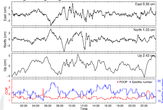
Figure 5-29 random walk constraint (0.0001 m/sqrt(s)) position sequence for abpo of 2024 001
