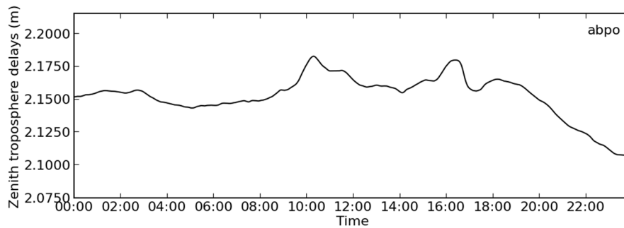
Figure 5-17 Example of plotztd.py
