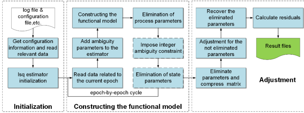
Figure 4-3 lsq algorithm flow. (The dashed box part is executed only when the ambiguity parameters is eliminated)
