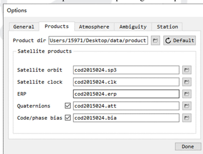
Figure 6-6 Using products of other AC
