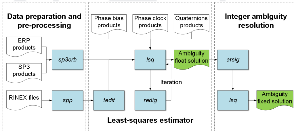
Figure 4-1 Program structure of PRIDE PPP-AR
