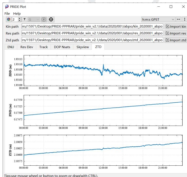
Figure 6-18 zdd, zwd and ztd-t charts
