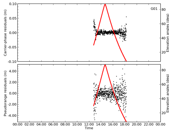
Figure 5-15 Example of plotres.py
