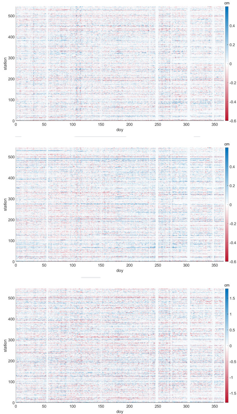
Figure B-1 Difference between PRIDE PPP-AR III solution and IGS SINEX solution of various stations.
