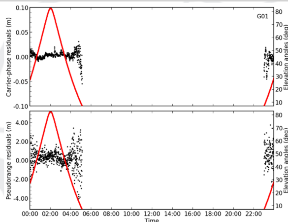
Figure 5-23 Residuals of abmf, 001 day in 2020
