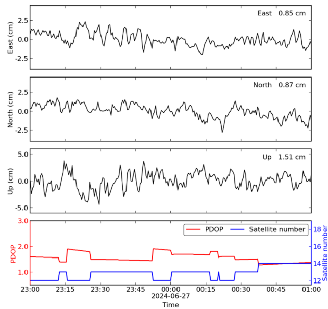
Figure 5-31 Time sequence plot of cross-day position on day 178-179 in 2024 of bamf (half-hourly results before and after the day boundary)
