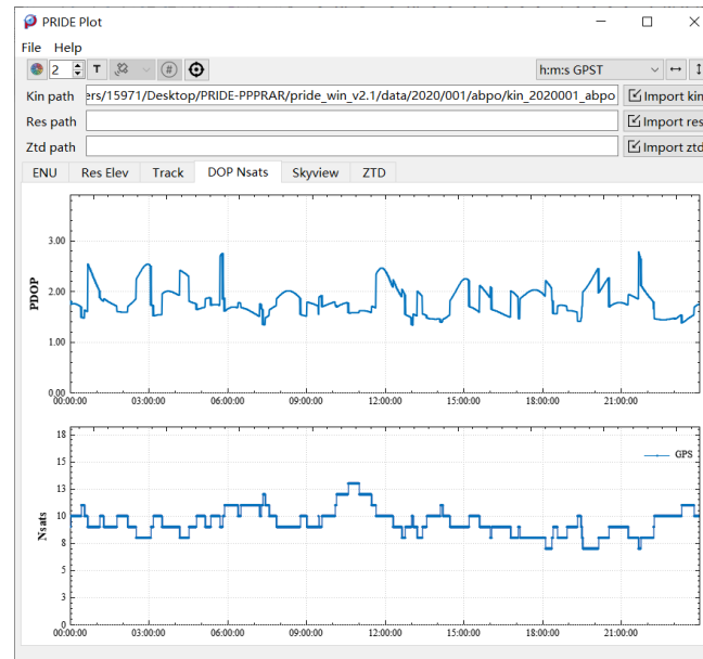
Figure 6-15 DOP and Nsats-t charts
