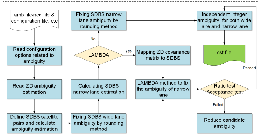
Figure 4-5. arsig algorithm flow. ZD indicates the zero difference
