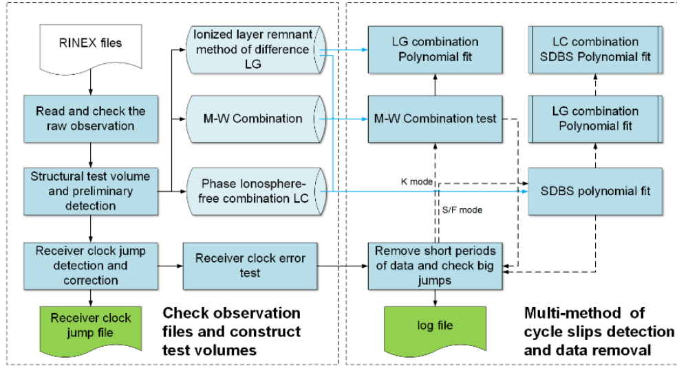
Figure 4-2 tedit algorithm flow. (The light blue columns indicate the constructed test volume; the blue line indicates the input of each test volume; the black dashed line indicates the running process controlled by the pdp3 script and the process is performed only once; SDBS indicates the single difference between satellites)
