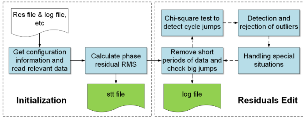
Figure 4-4 redig algorithm flow. The black dashed line indicates that the process is executed only once
