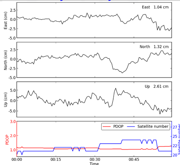
Figure 5-26 Position time series of ccj2, 210 day in 2021
