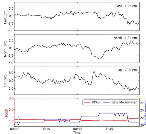
Figure 5-24 Position time series of ccj2, 210 day in 2021
