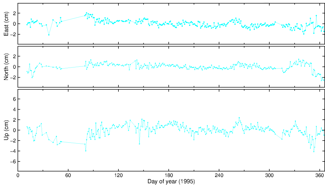
Figure C-1 Position time series at station ALBH in 1995
