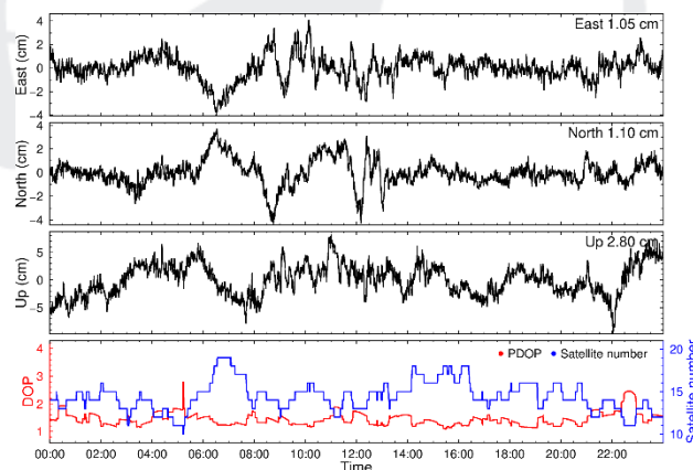
Figure 5-30 kinematic position sequence for abpo of 2024 001
