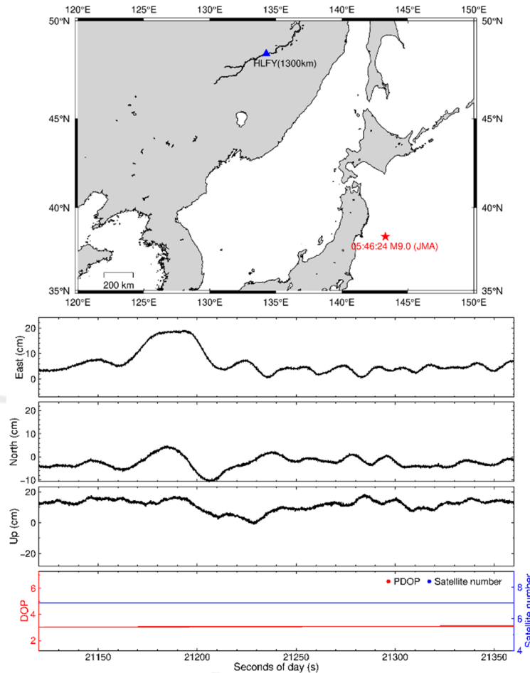
Figure B-2 Time series of super-high-rate kinematic solutions (cm) in east, north, and up components at station HLFY on March 11, 2011
