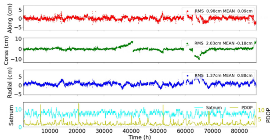
Figure 5-28 Time series diagram of grace satellite's resolution accuracy on the 1 day of 2023
