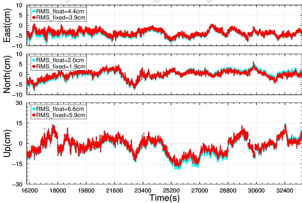
Figure B-4 Location differences between PRIDE PPP-AR and WayPoint software
